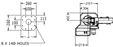
MOUNTING BASE PATTERN
